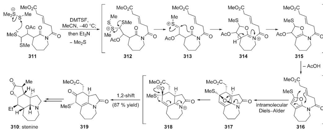
Scheme 43. A heterocyclization/Diels-Alder reaction/rearrangement cascade in the total synthesis of stenine ( 310 ; Ginn and Padwa, 2002). [162]
